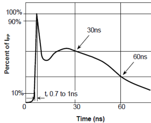
Fig.4 Pulse Waveform-ESD(IEC61000-4-2)
