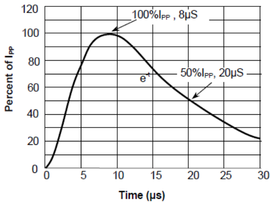
Fig.3 Pulse Waveform-8/20μs
